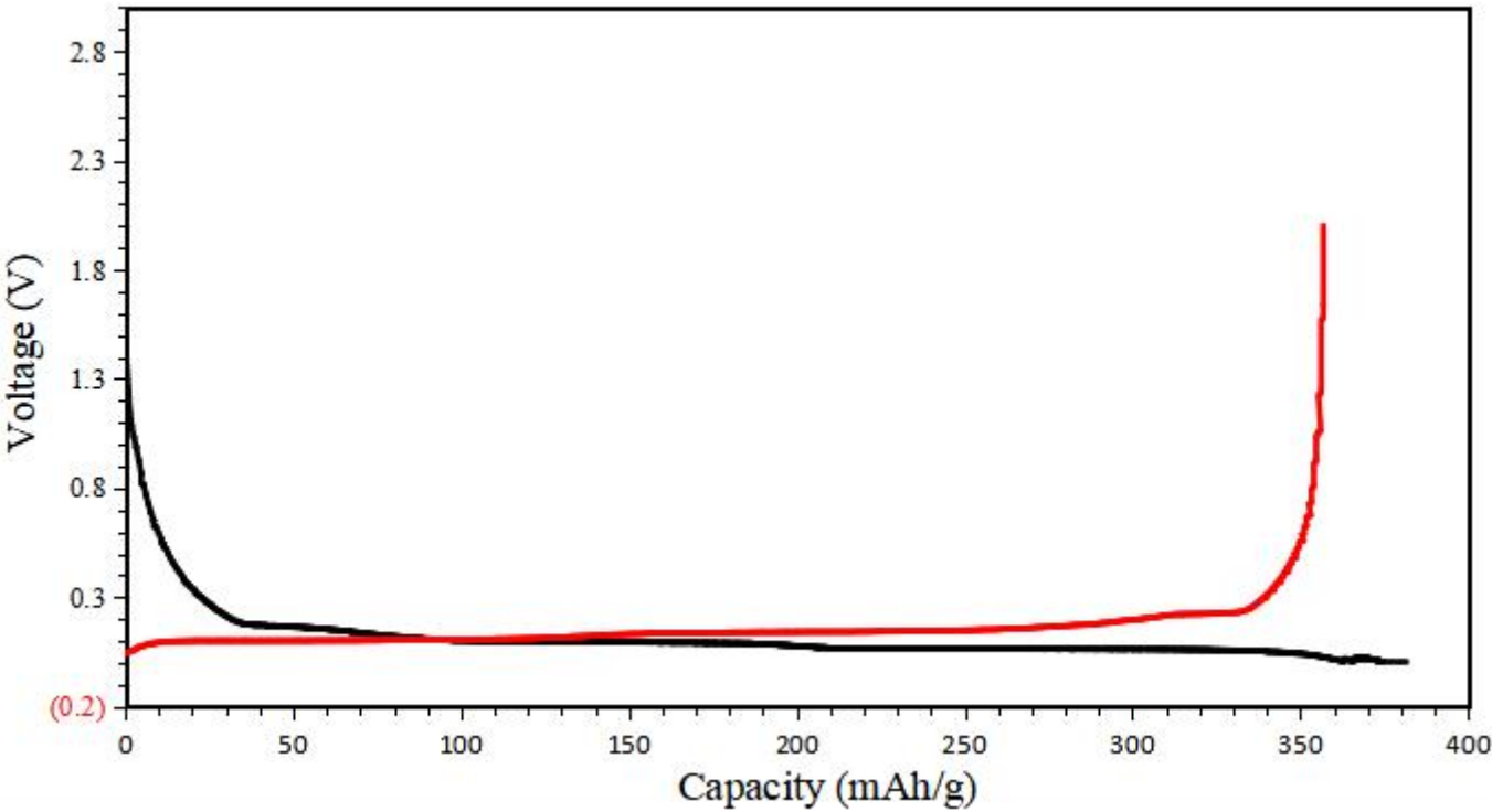
充放电曲线 Charge-Discharge Curves
