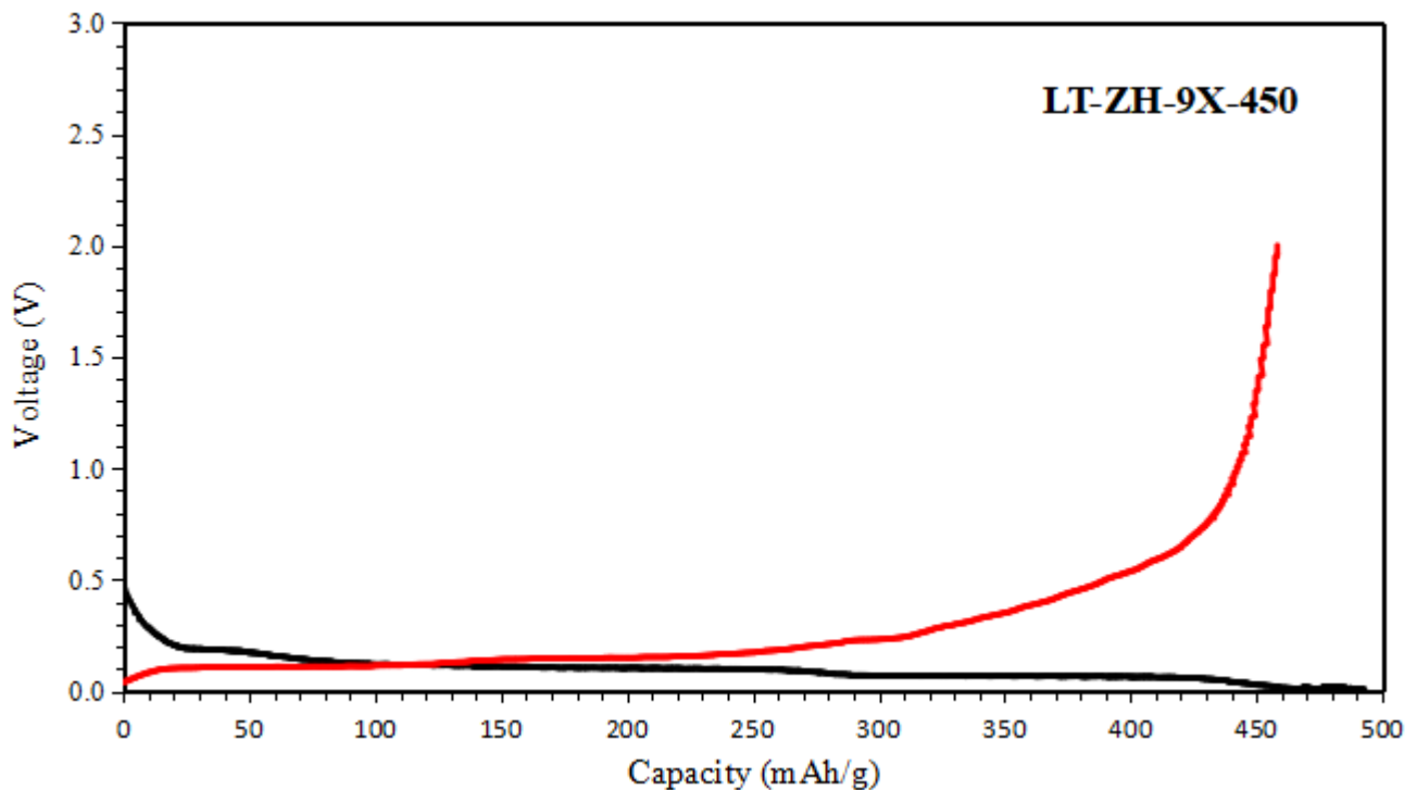
Charge-Discharge Curves
