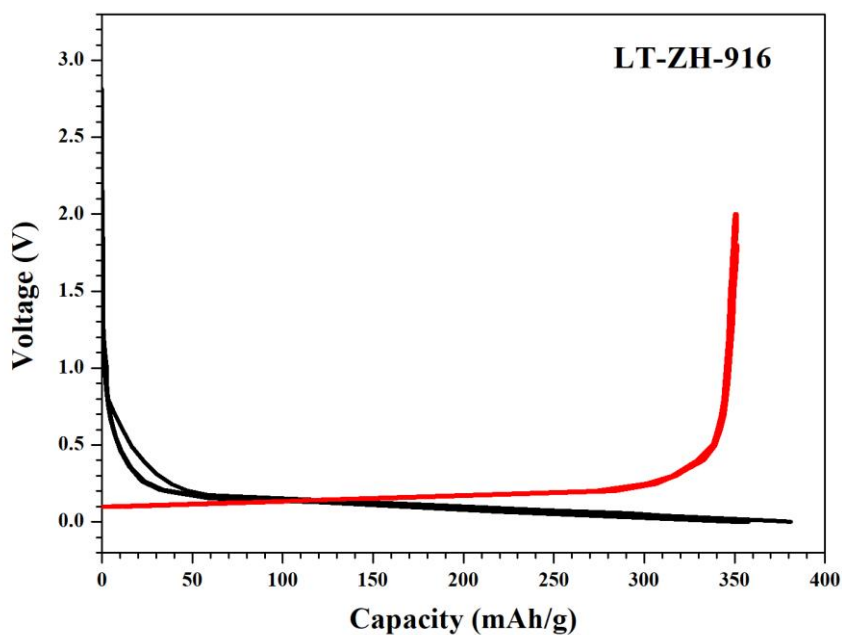
Charge-Discharge Curves
