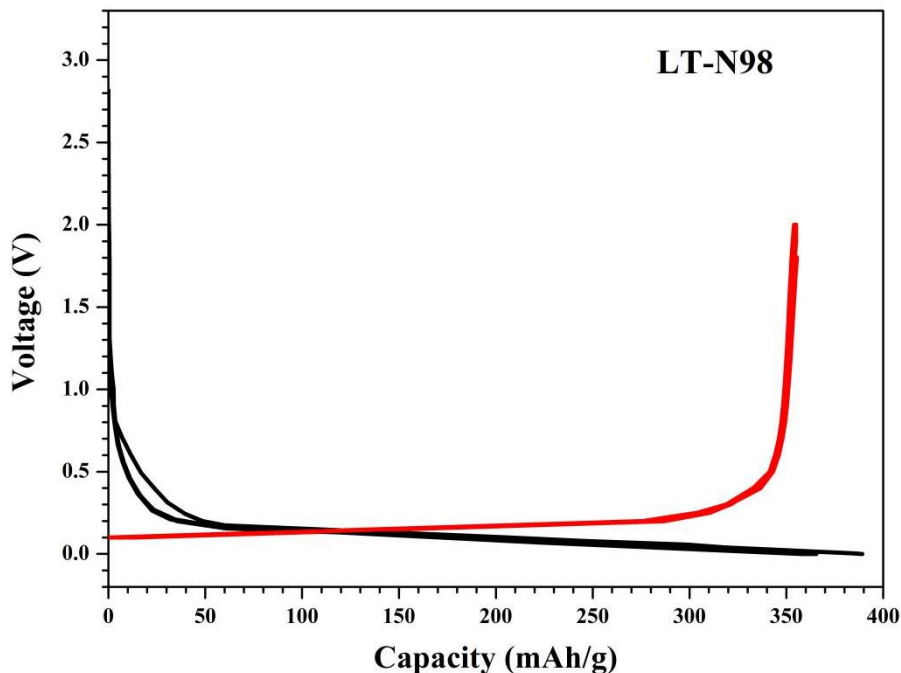
Charge-Discharge Curves
