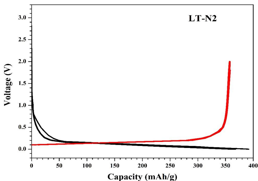
Charge-Discharge Curves
