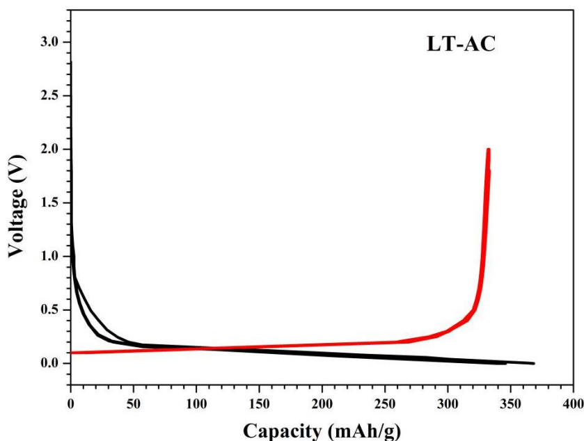
Charge-Discharge Curves
