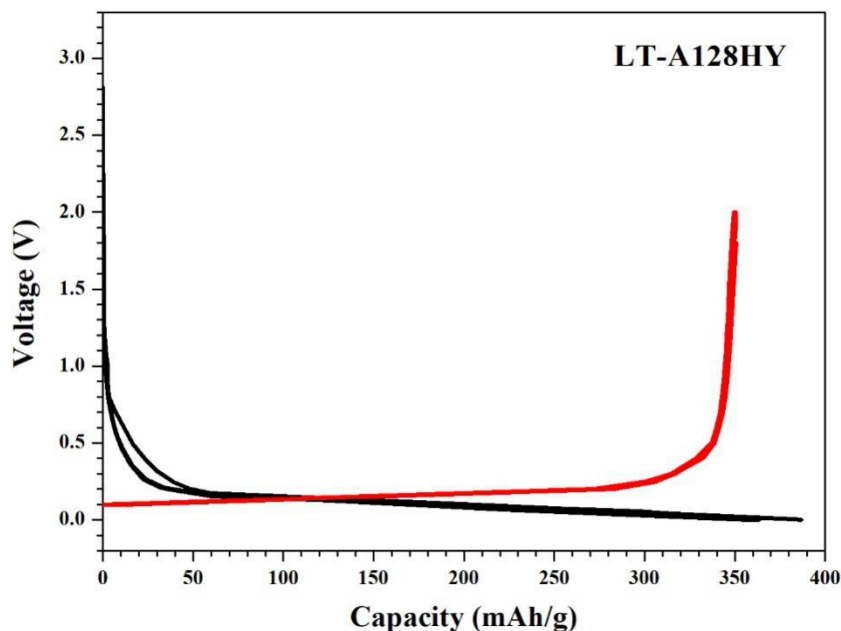
Charge-Discharge Curves
