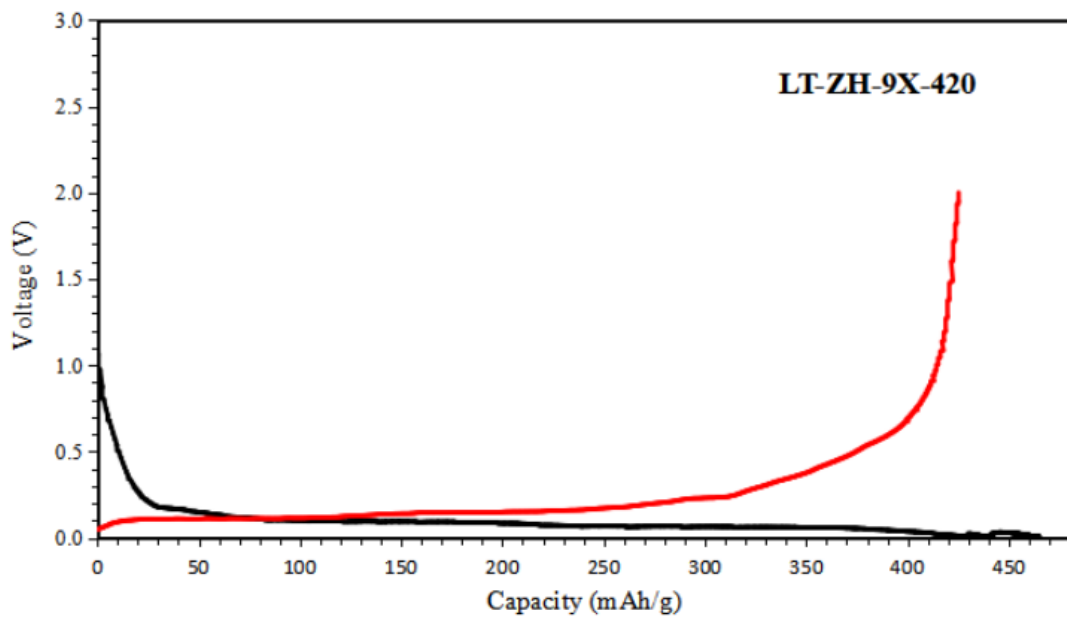
Charge-Discharge Curves
