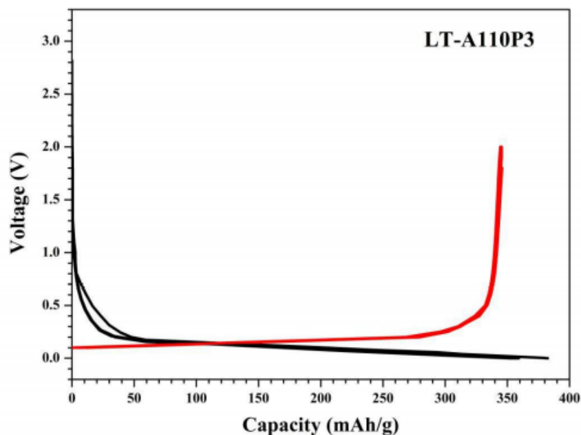
Charge-Discharge Curves
