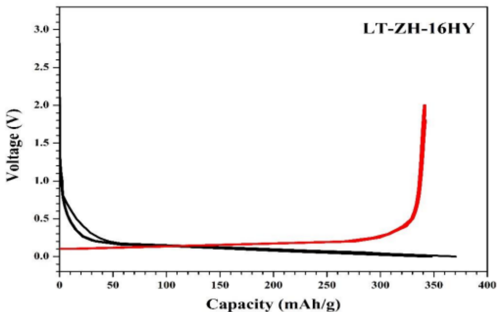
Charge-Discharge Curves
