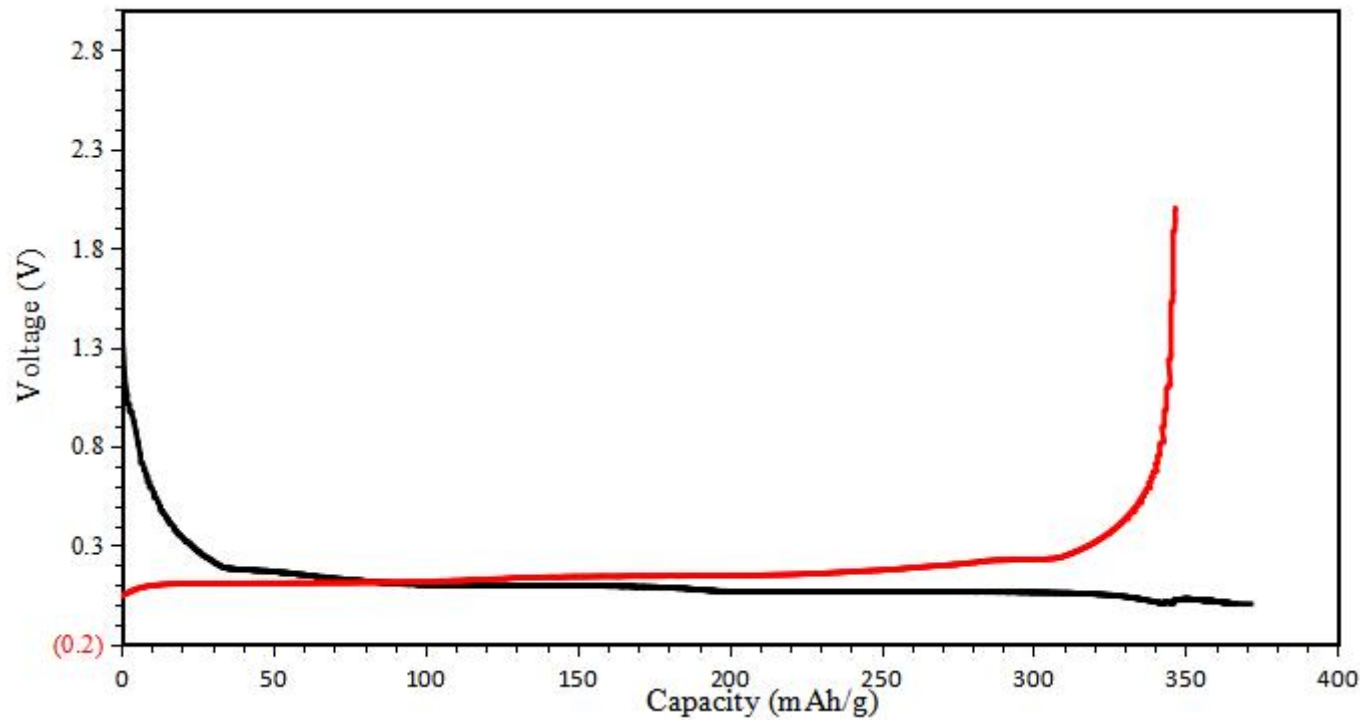
充放电曲线 Charge-Discharge Curves
